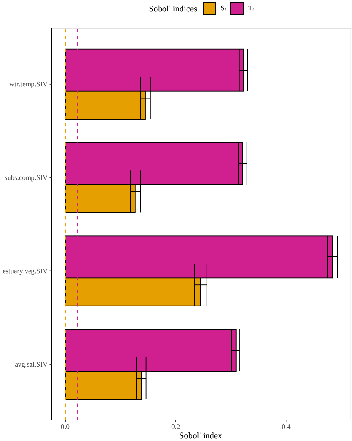
Figure 6. Results of a sensitivity analysis for the brownshrimpNGulfofMex model based on a limiting factor structure. Dashed lines represent baseline numerical approximation error for S_i and T_i ( i.e. , dummy variables).
