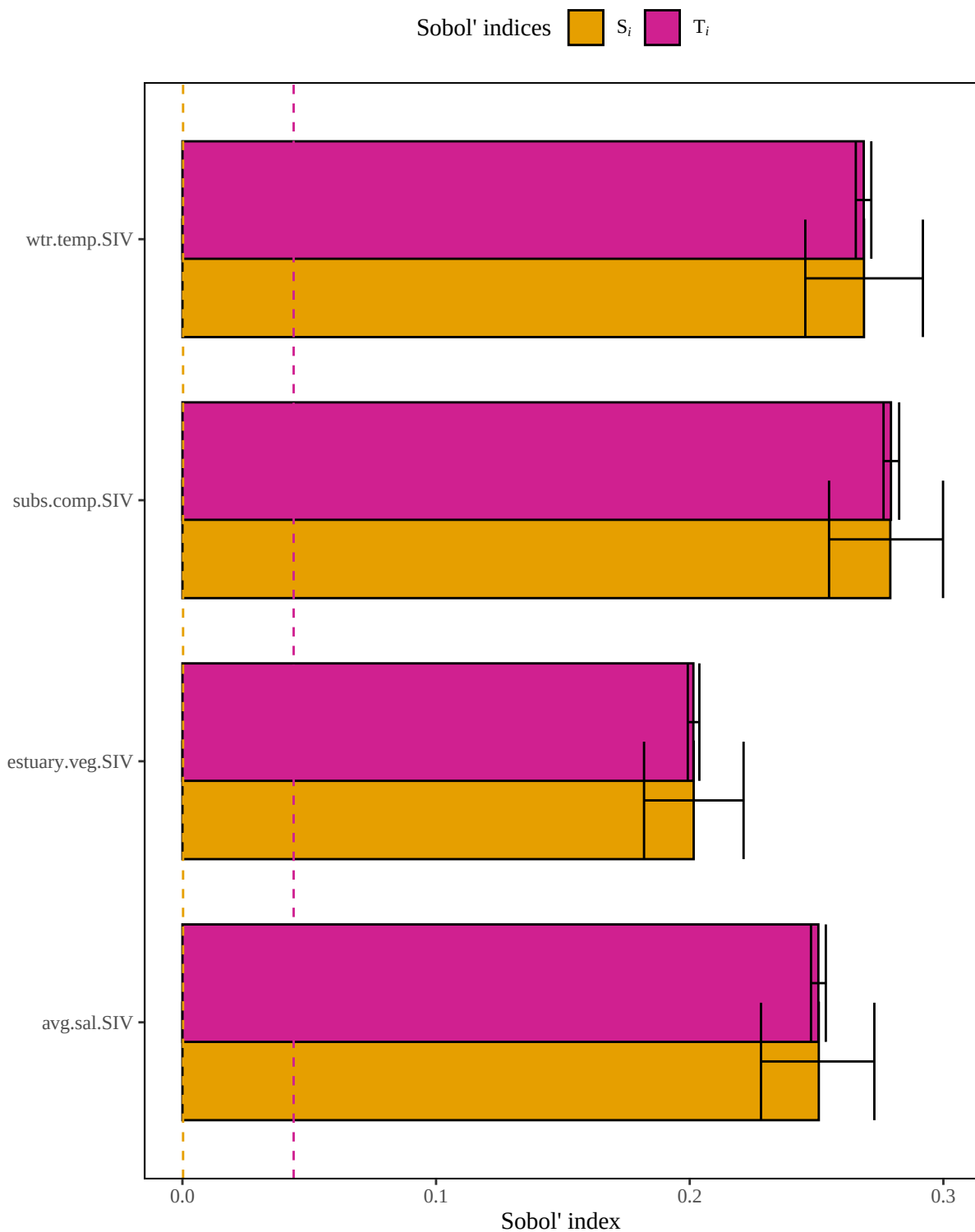
Figure 4. Results of a sensitivity analysis for the brownshrimpNGulfofMex model based on an arithmetic mean structure. Dashed lines represent baseline numerical approximation error for S_i and T_i ( i.e. , dummy variables).
