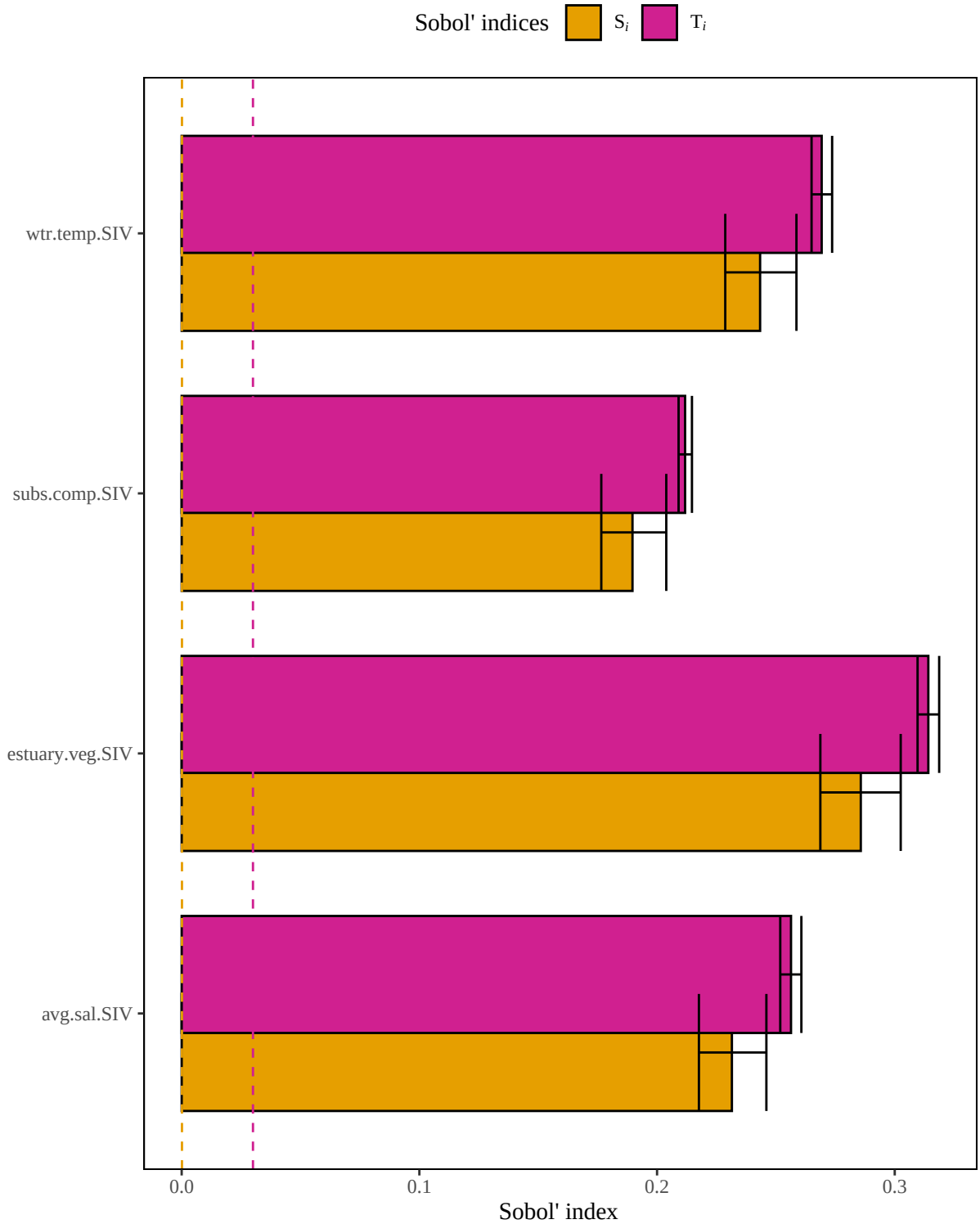
Figure 5. Results of a sensitivity analysis for the brownshrimpNGulfofMex model based on a geometric mean structure. Dashed lines represent baseline numerical approximation error for S_i and T_i ( i.e. , dummy variables).
