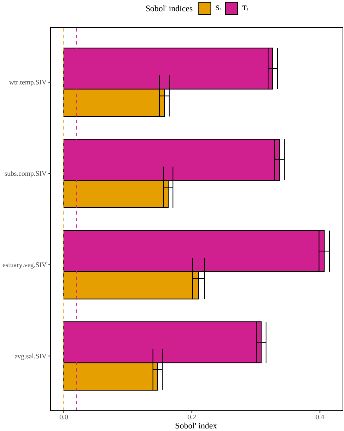
Figure 7. Results of a sensitivity analysis for the brownshrimpNGulfofMex model based on a multiplicative mean structure. Dashed lines represent baseline numerical approximation error for S_i and T_i ( i.e. , dummy variables).
